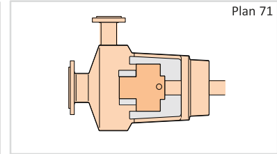
Tapped connections for the purchaser's use, e.g., for future use of buffer gas.
