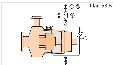
Barrier fluid system pressurized by a bladder accumulator supplying clean liquid for an arrangement 3 pressurized dual seal.
