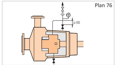
A containment seal chamber drain for non-condensing leakage on arrangement 2 unpressurized seals with containment seals (2CW-CS and 2NC-CS). Used if the pumped fluid does not condense at ambient temperatures.
