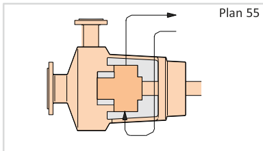
Unpressurized external buffer fluid system supplying clean buffer liquid for the outer seal of an arrangement 2 unpressurized dual seal. Buffer liquid is supplied by an external pump or pressure system.
