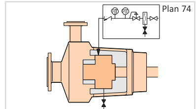
Externally supplied barrier gas for arrangement 3 dual pressurized non-contacting gas seals (3NC-FB, 3NCBB, 3NC-FF).
