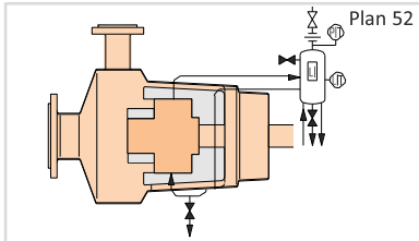
Reservoir providing buffer liquid for the outer seal of an arrangement 2 unpressurized dual seal. The buffer liquid
