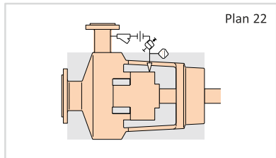
Recirculation from the pump discharge through a strainer and a flow control orifice and a cooler into the seal chamber.
