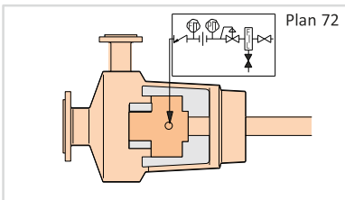
Externally supplied buffer gas for arrangement 2 unpressurized seals with dry running containment seal (2CW-CS and 2NC-CS). Buffer gas is maintained at a pressure less than seal chamber pressure. The buffer gas pressure should not exceed 0.7 bar (10 PSI)
