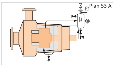
Pressurized barrier fluid reservoir supplying clean fluid for an arrangement 3 pressurized dual seal.
