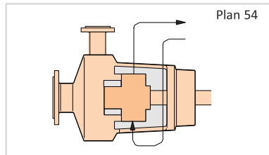
Pressurized external barrier fluid system supplying clean liquid for an arrangement 3 pressurized dual seal. The barrier liquid is maintained at a pressure greater than seal chamber pressure and is circulated by an external pump or pressure system.
