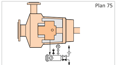
A containment seal chamber leakage collection system for condensing or mixed phase leakage on arrangement 2 unpressurized seals with containment seals (2CW-CS and 2NC-CS).
